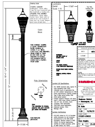
Proposed Luminaire Detail
